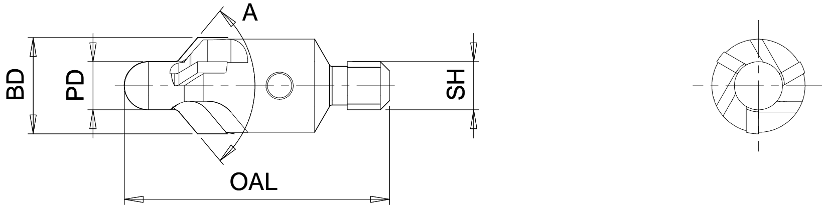
PCD 3fl Countersink Integral Pilot (mm)
