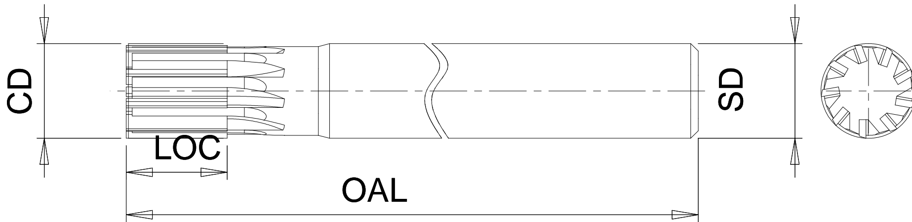
PCD Multiflue End-mill (Inch)
