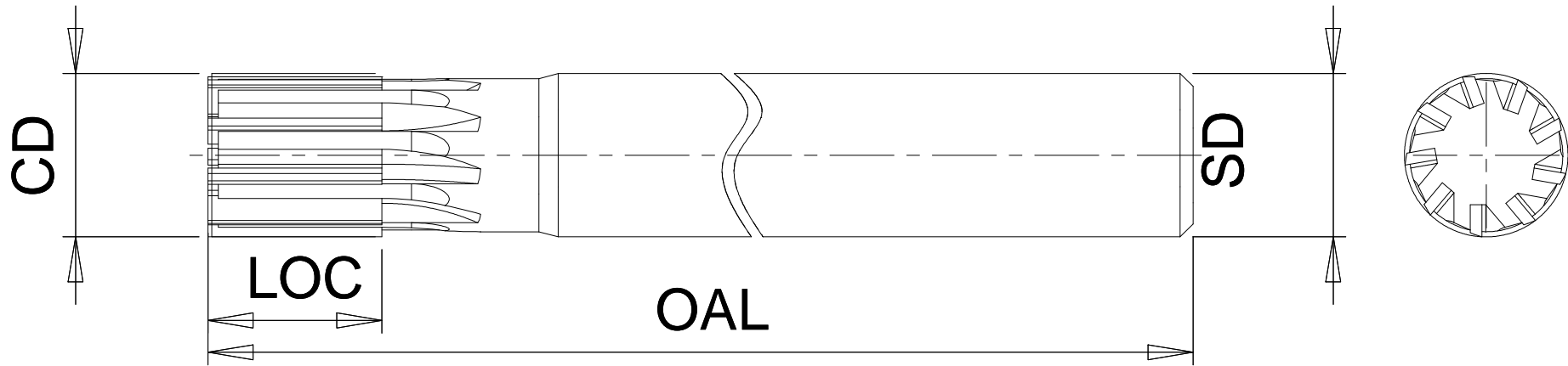
PCD Multiflute End-mill (mm)
